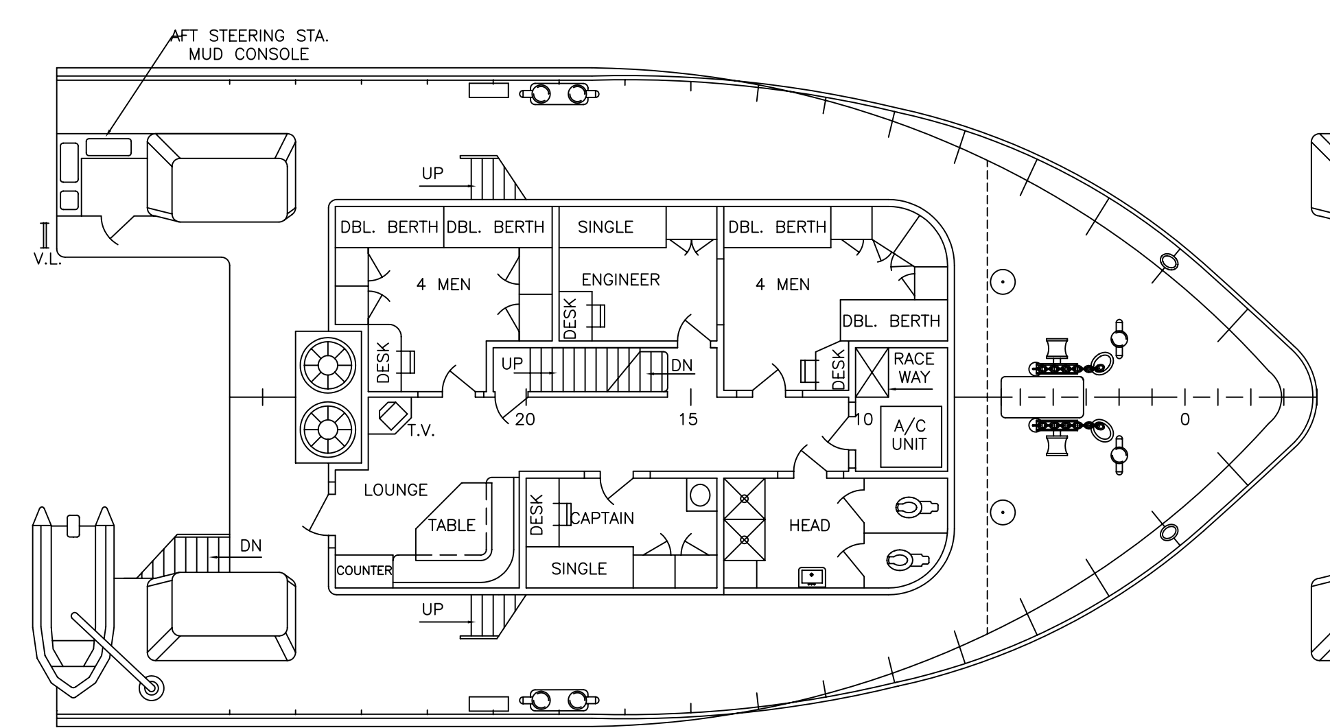
FOCSLE DECK 25'-11 3/4" ABOVE BASELINE
