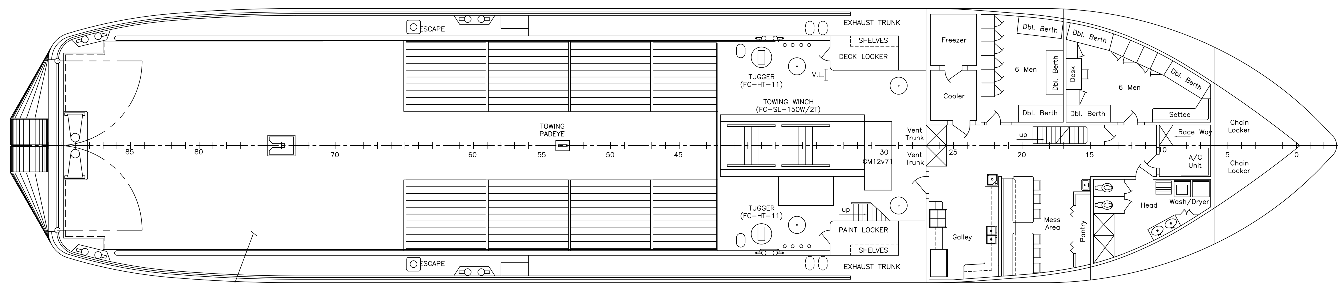
MAIN DECK 14'-0" ABOVE BASELINE
