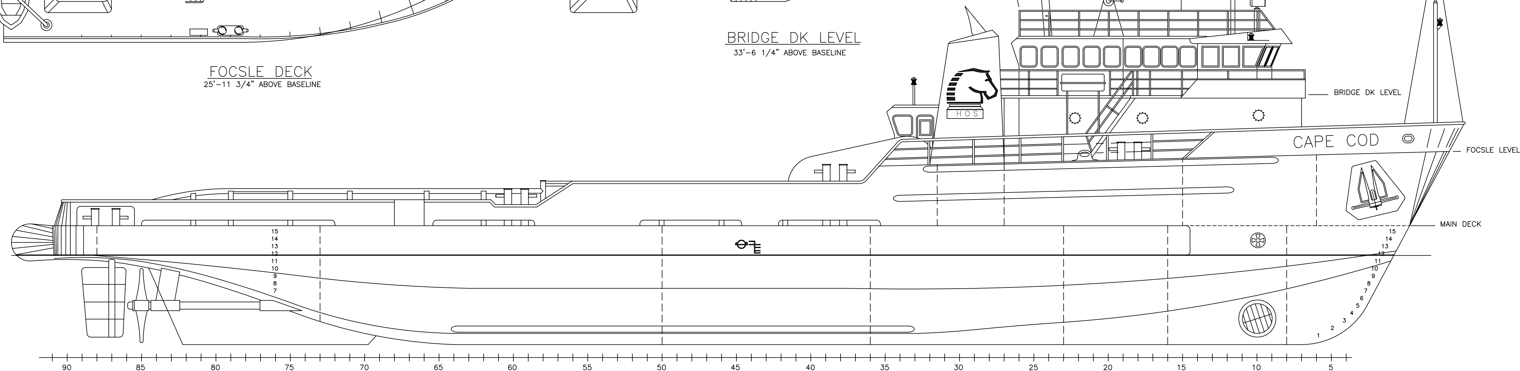
OUTBOARD PROFILE
