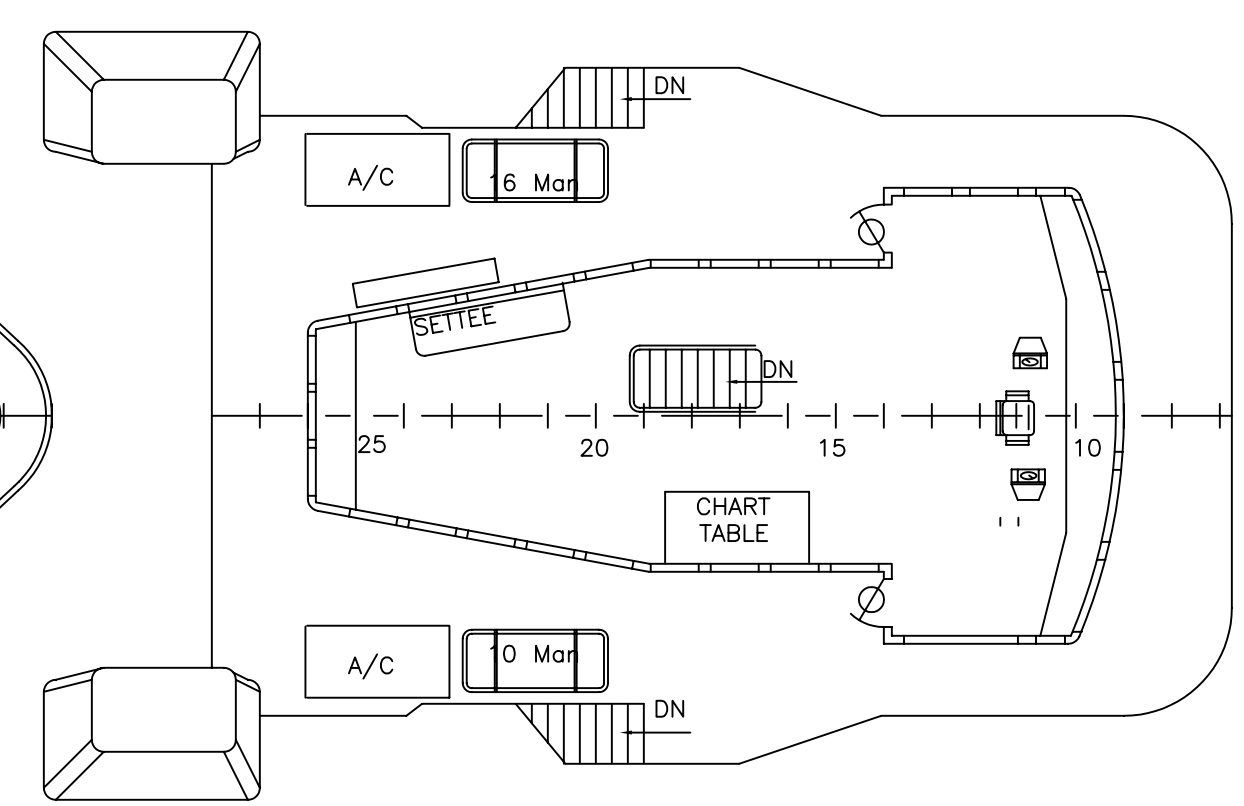
BRIDGE DK LEVEL 33'-6 1/4" ABOVE BASELINE
