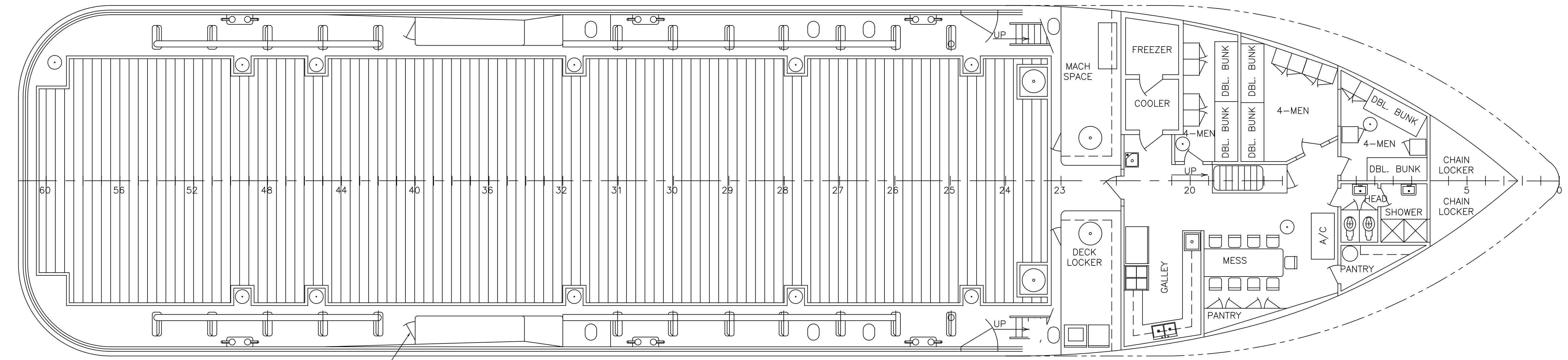
MAIN DECK 13'-0" ABOVE BASELINE
