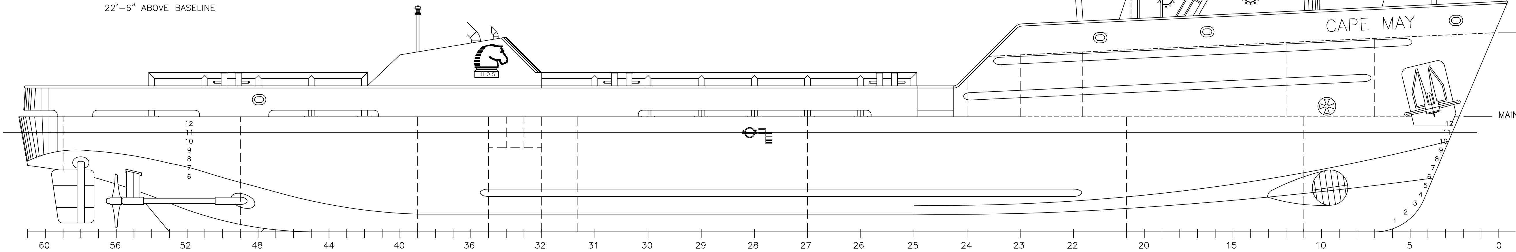
OUTBOARD PROFILE
