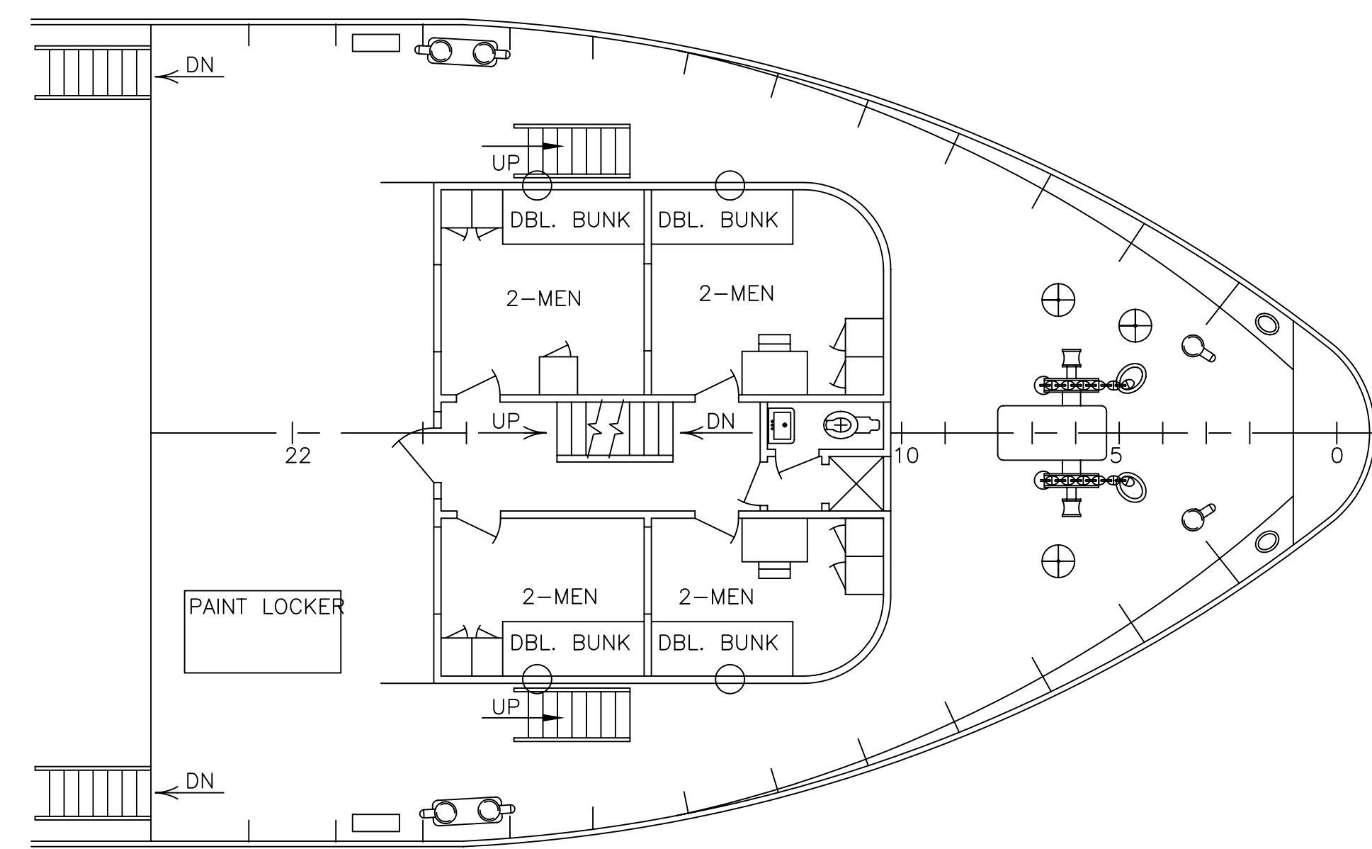
FOCSLE DECK 22'-6" ABOVE BASELINE
