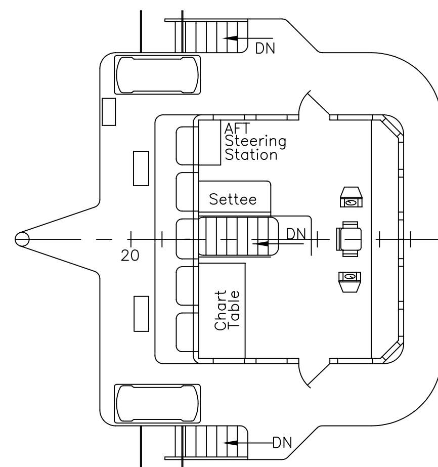
BRIDGE DK LEVEL 29'-3" ABOVE BASELINE
