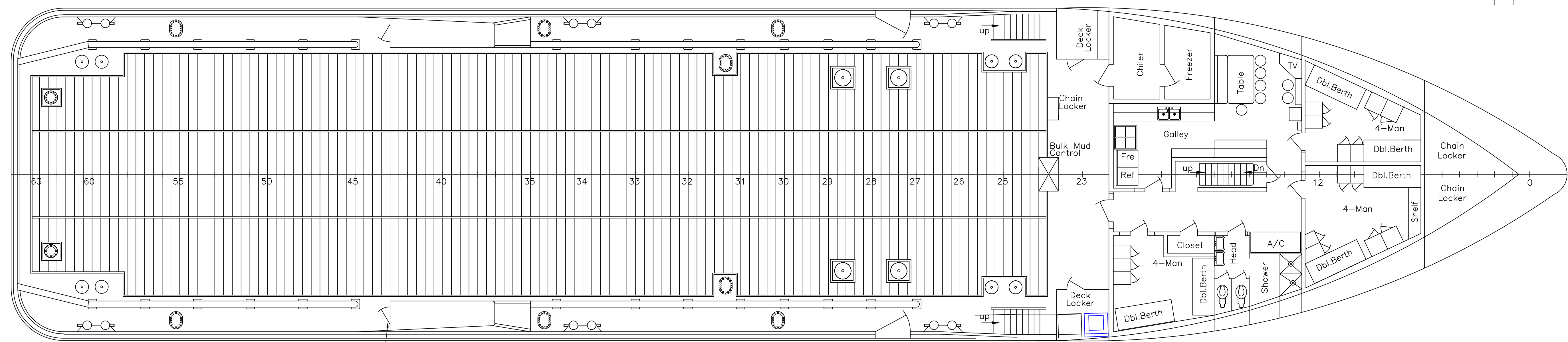
MAIN DECK 14'-0" ABOVE BASELINE
