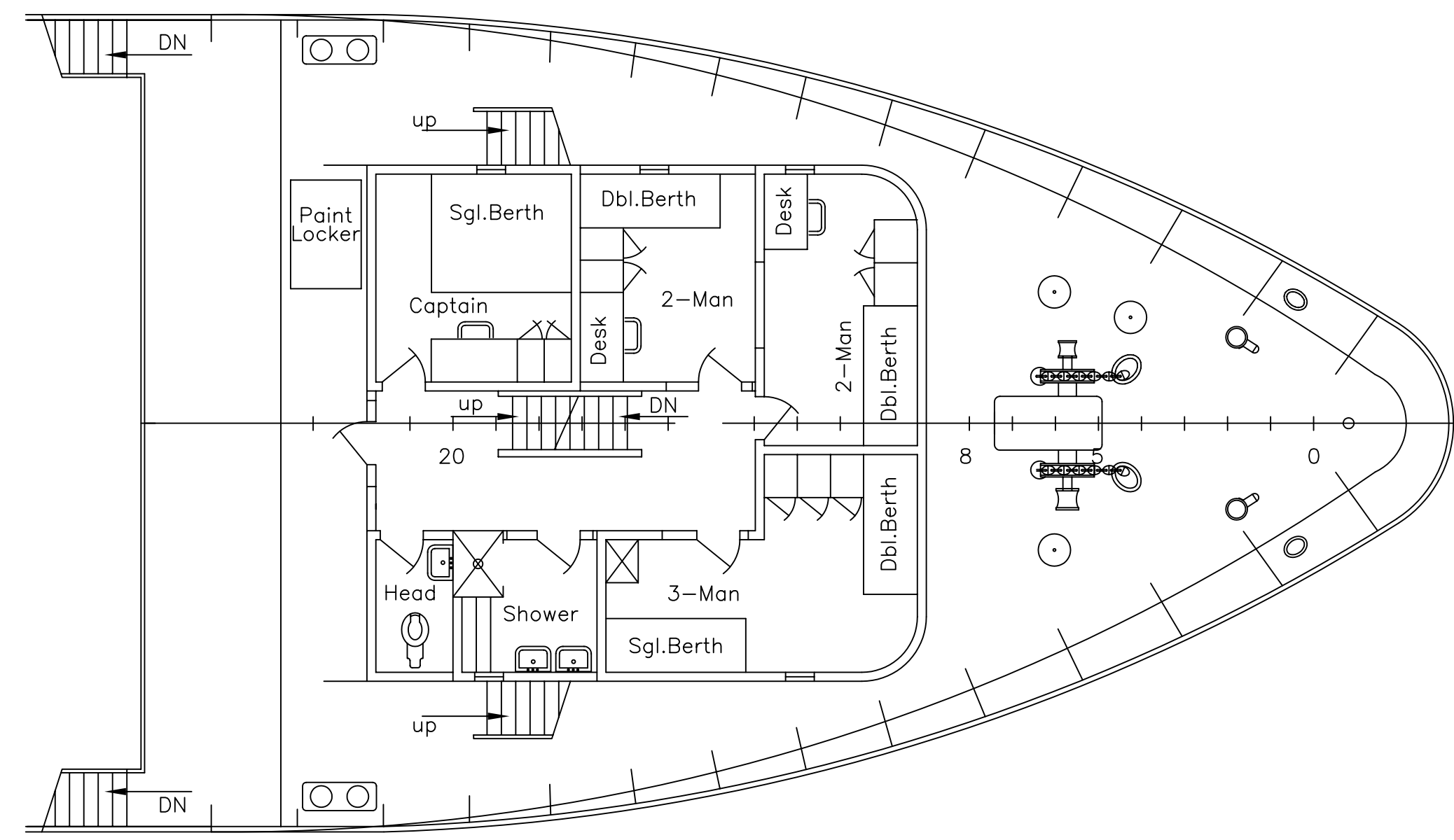
FOCSLE DECK 23'-11 7/8" ABOVE BASELINE
