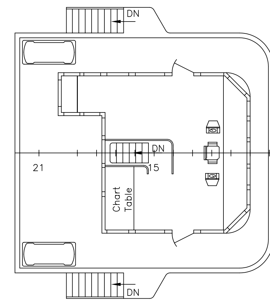
BRIDGE DK LEVEL 30'-10 3/4" ABOVE BASELINE
