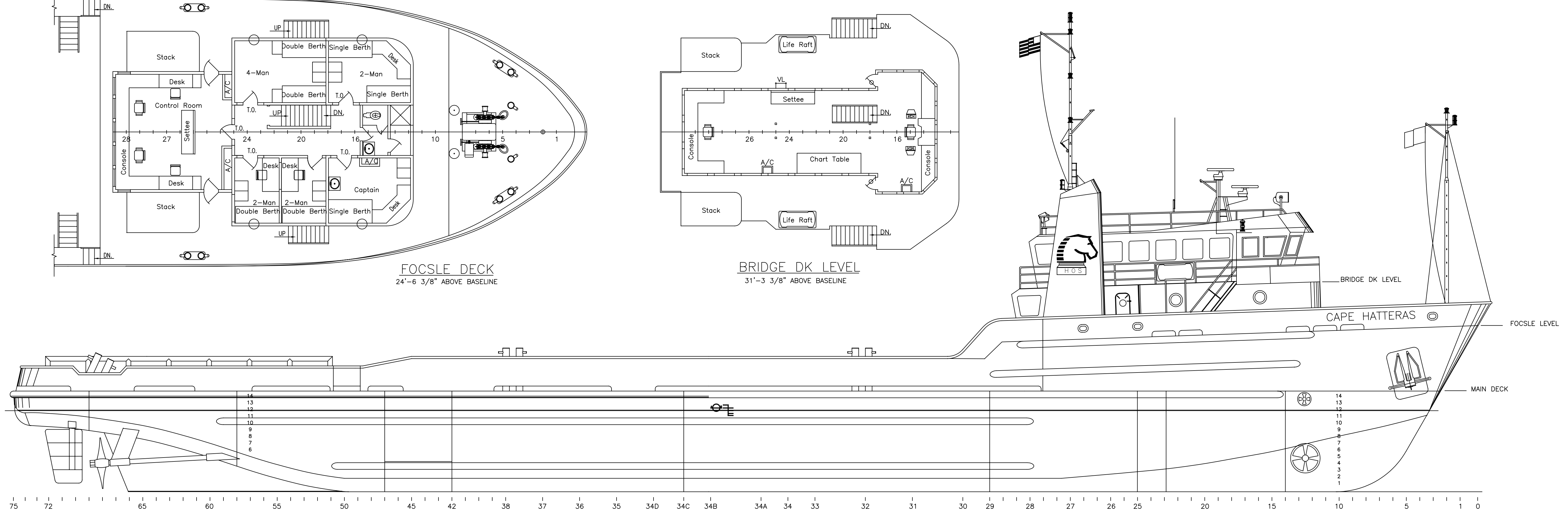
OUTBOARD PROFILE
