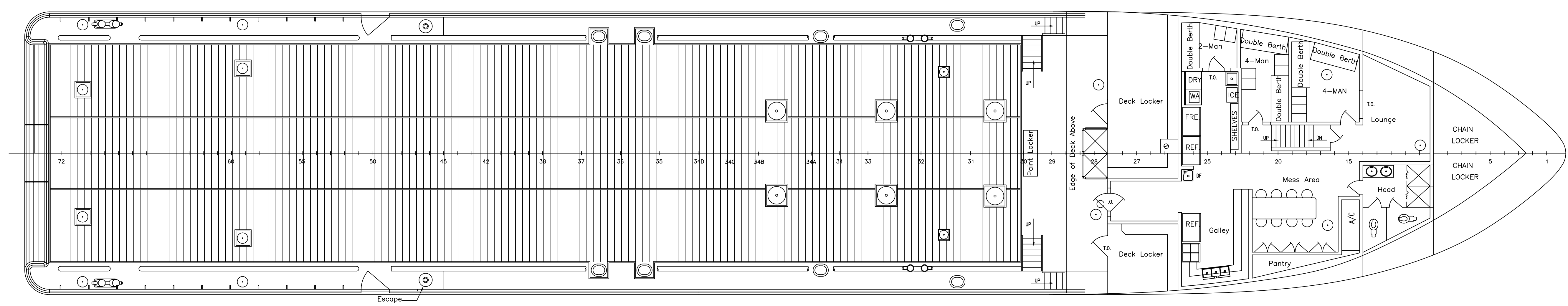
MAIN DECK 14'-0" ABOVE BASELINE
