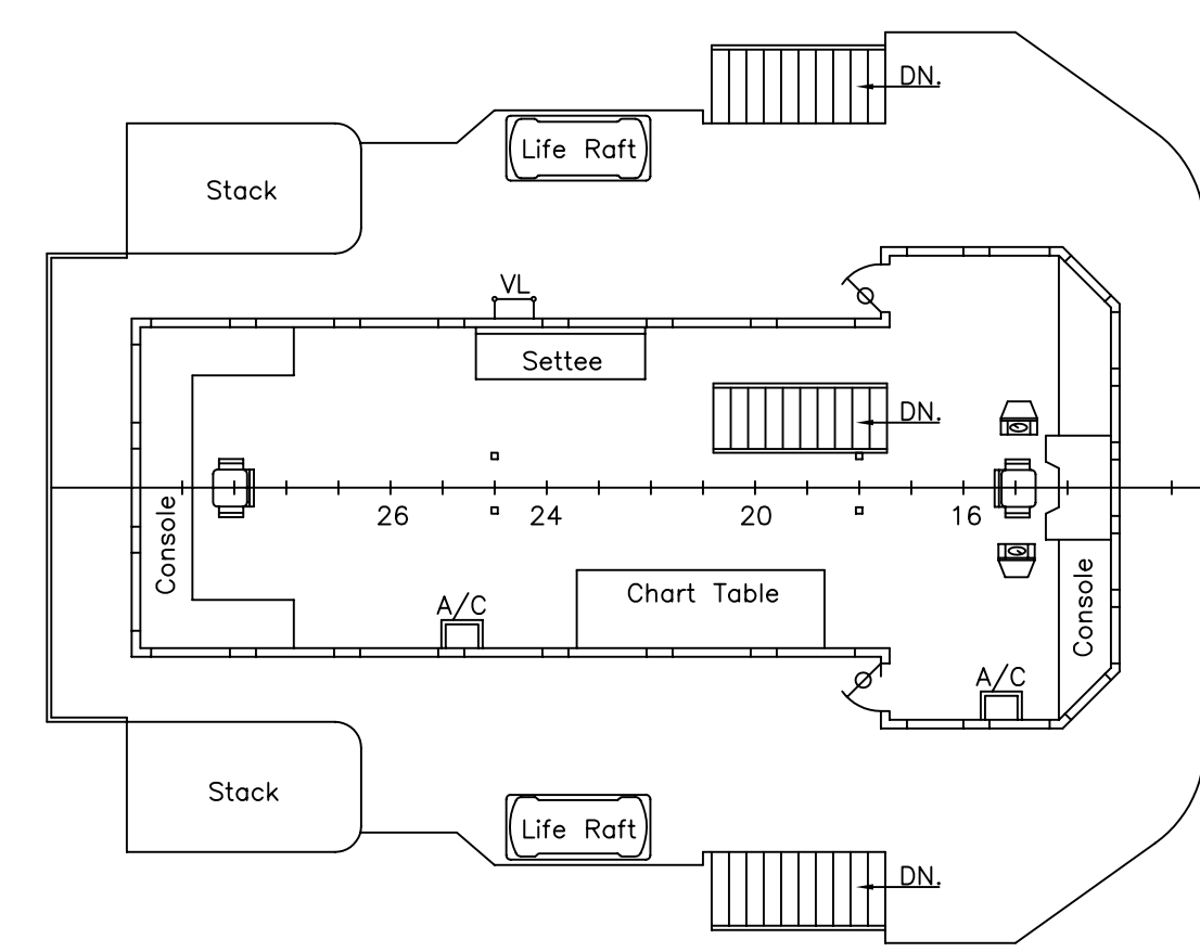
BRIDGE DK LEVEL 31'-3 3/8" ABOVE BASELINE
