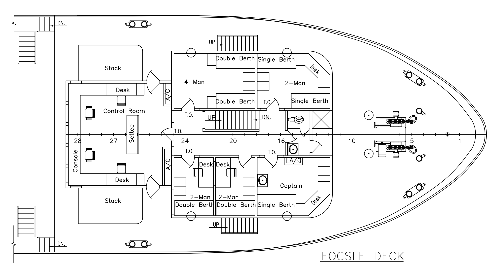
FOCSLS DECK 24'-6 3/8" ABOVE BASELINE
