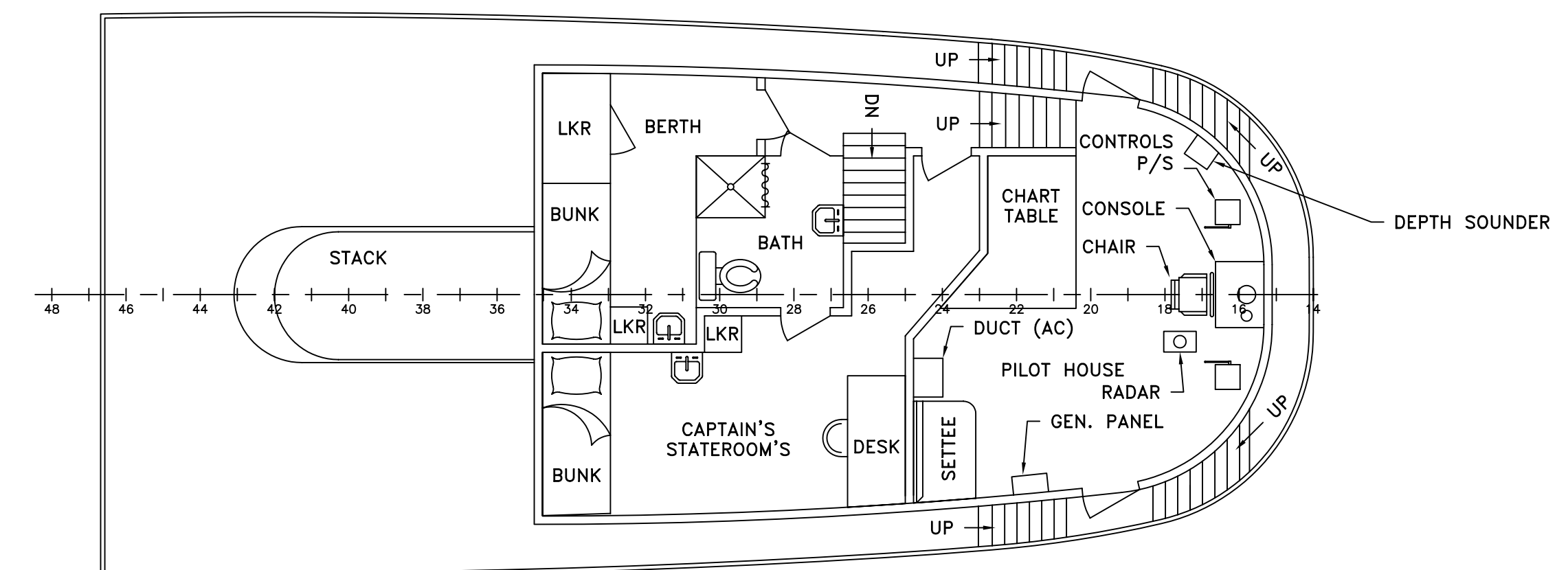
PILOT HOUSE DECK SCALE: 3/16"=1'-0"
