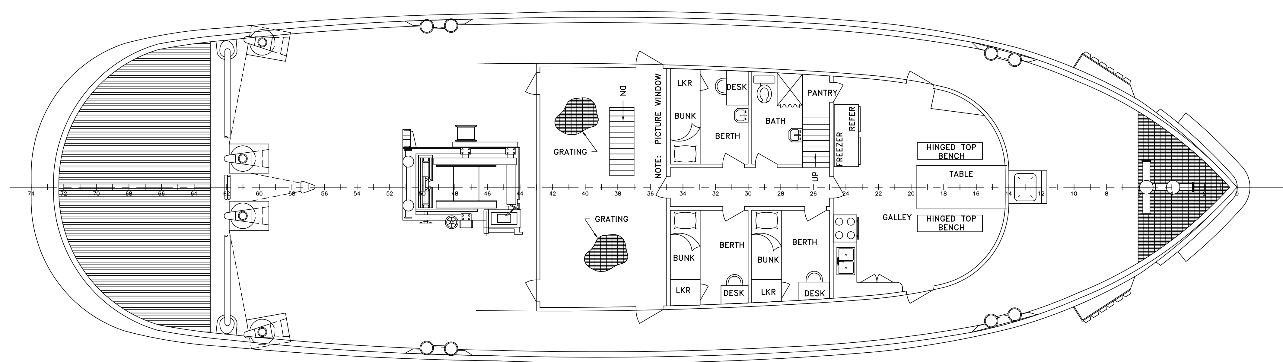
MAIN DECK SCALE: 3/16"=1'-0"
