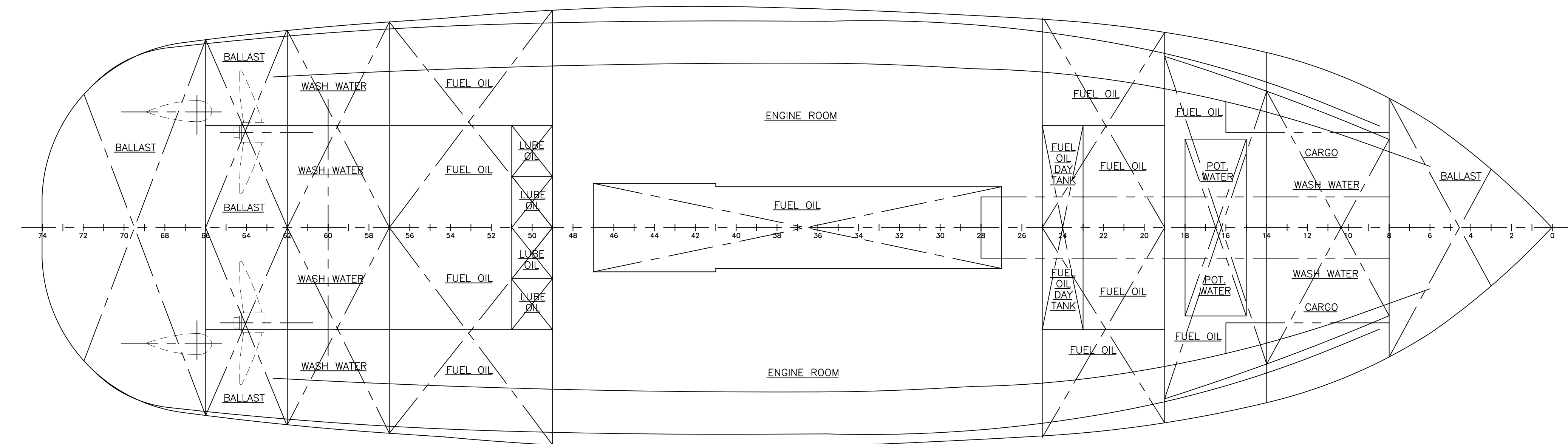
HOLD PLAN SCALE: 3/16"=1'-0"
