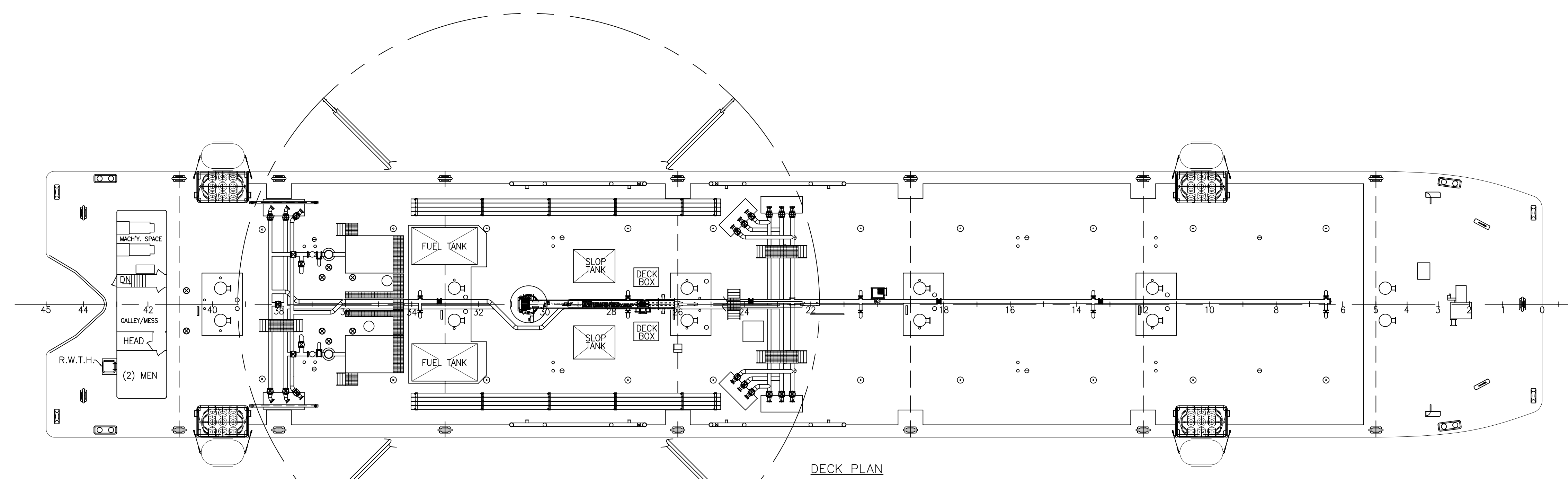
DECK PLAN
