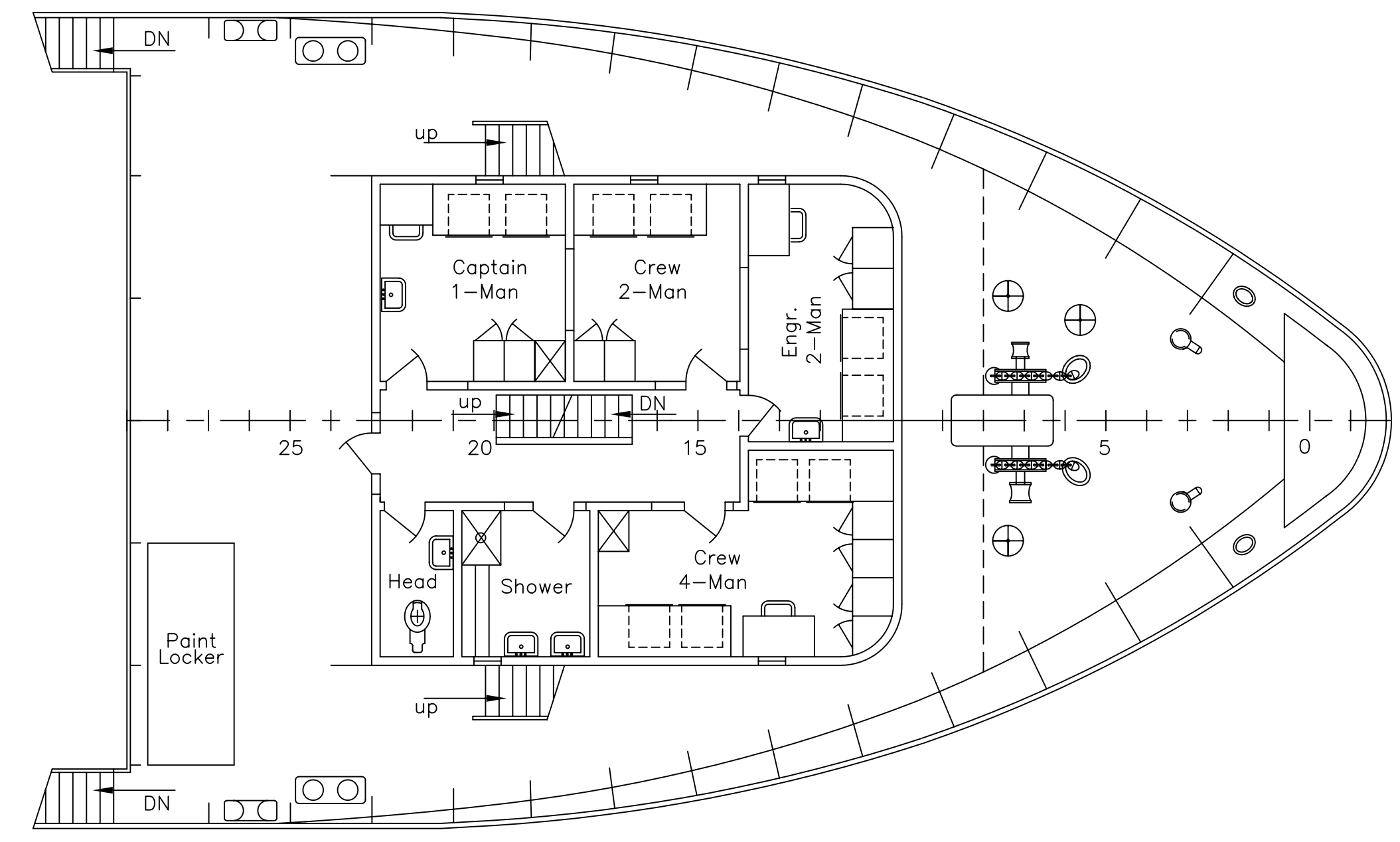
FOCSLE DECK 24'-0 3/8" ABOVE BASELINE
