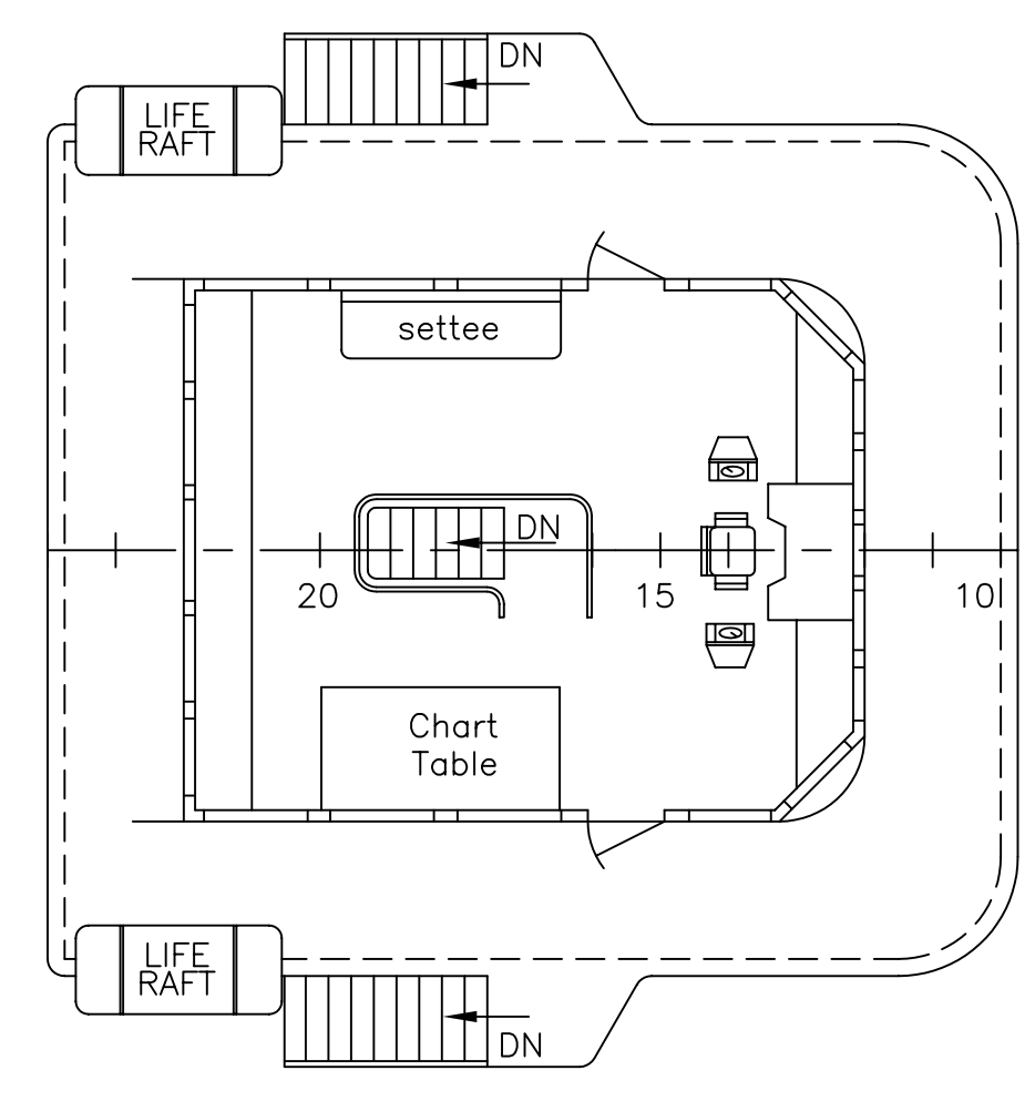
BRIDGE DK LEVEL 30'-7 5/8" ABOVE BASELINE
