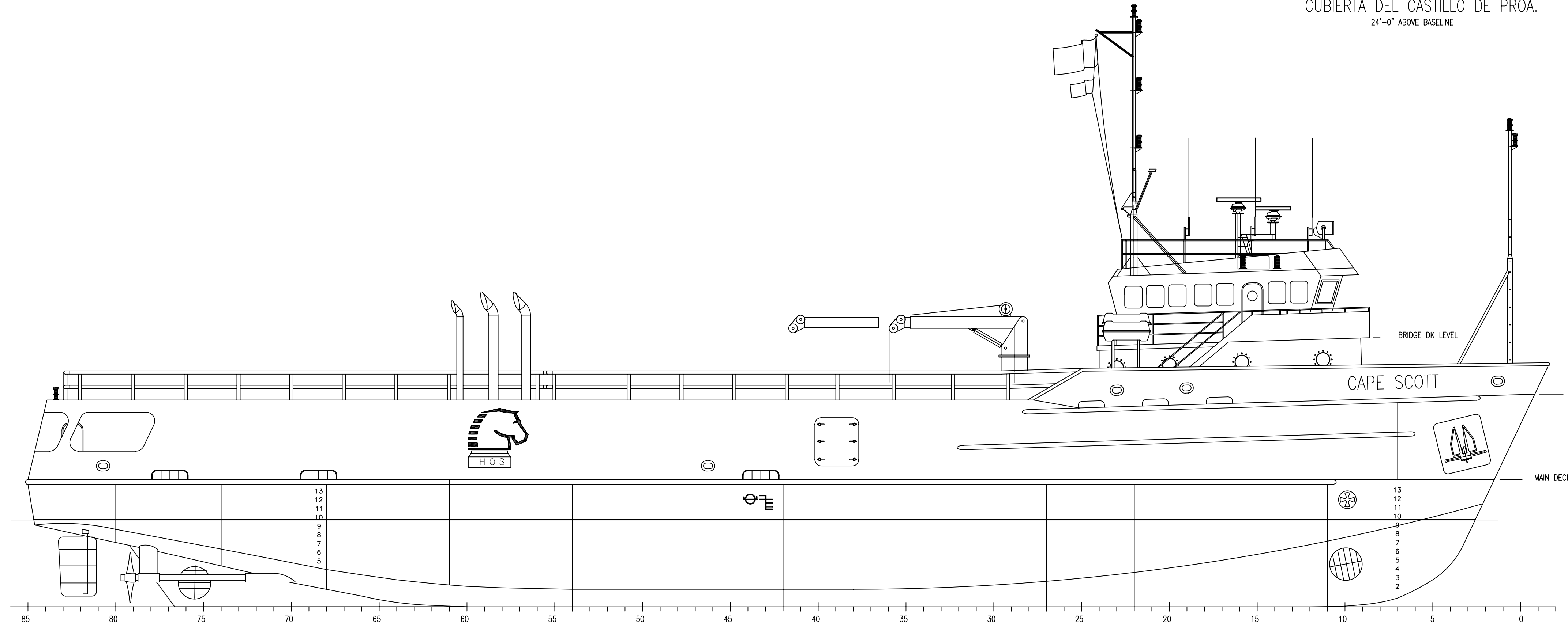
OUTBOARD PROFILE PERFIL
