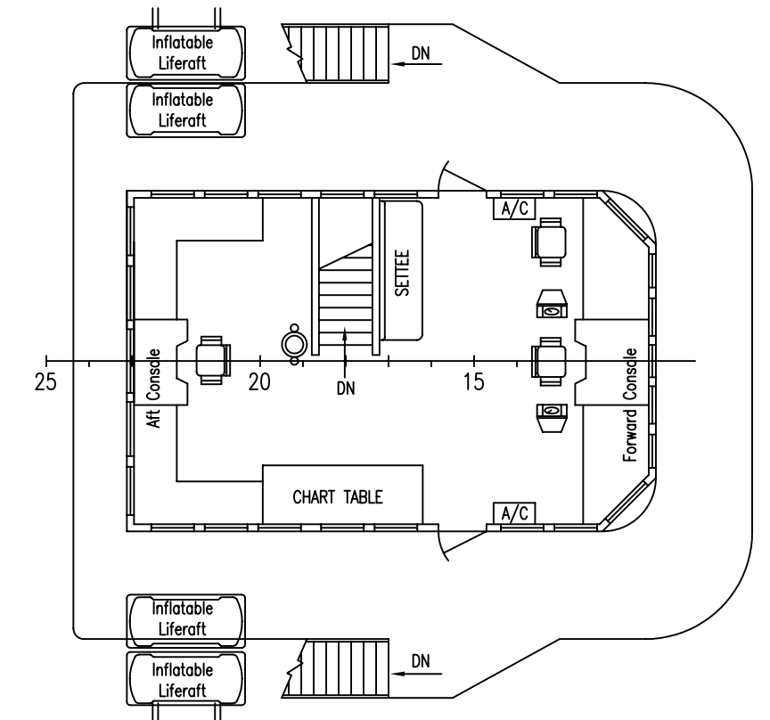
WHEELHOUSE PUENTE 30'-5" ABOVE BASELINE
