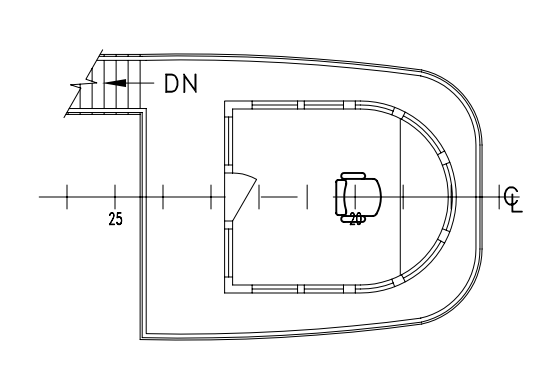
UPPER PILOTHOUSE DECK SCALE: 1/8"=1'-0"
