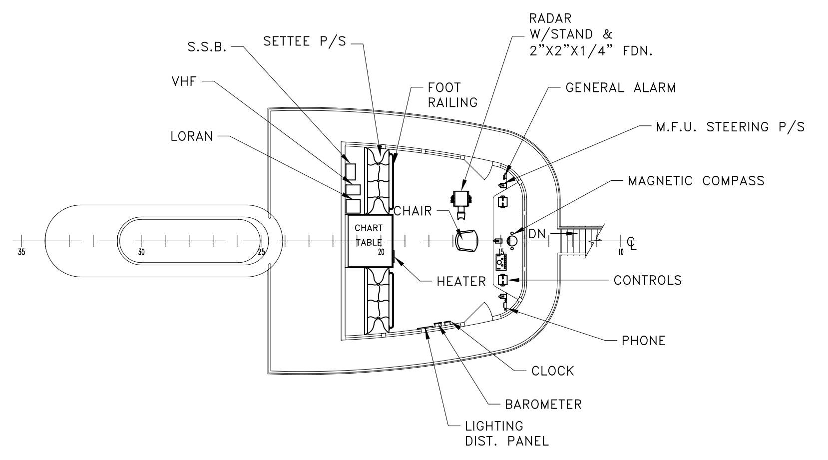
PILOTHOUSE DECK SCALE: 3/16"=1'-0"
